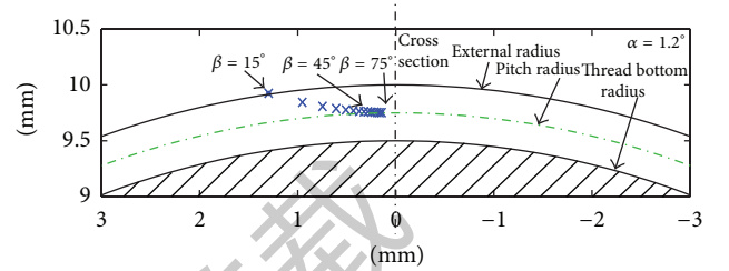
FIGURE 11: Meshing points under different vertex angle conditions.
